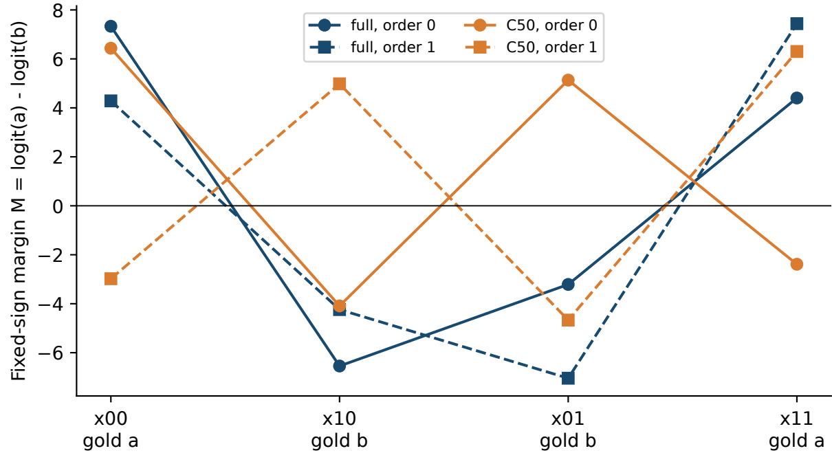
(b) C50: order dominates the queried child
