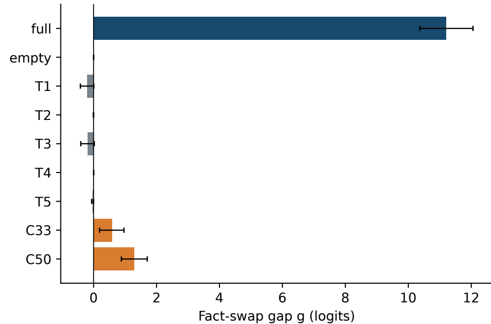
(a) Retention: 20 discovery families
